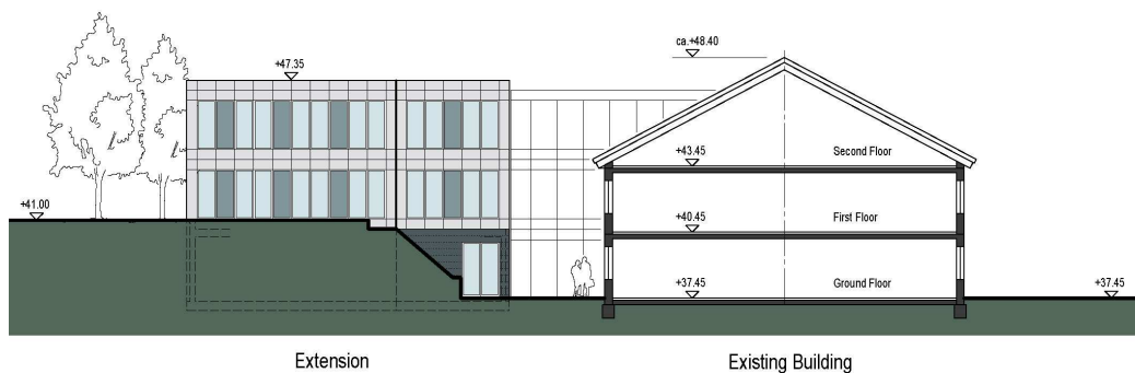
SECTION C - EAST ELEVATION
