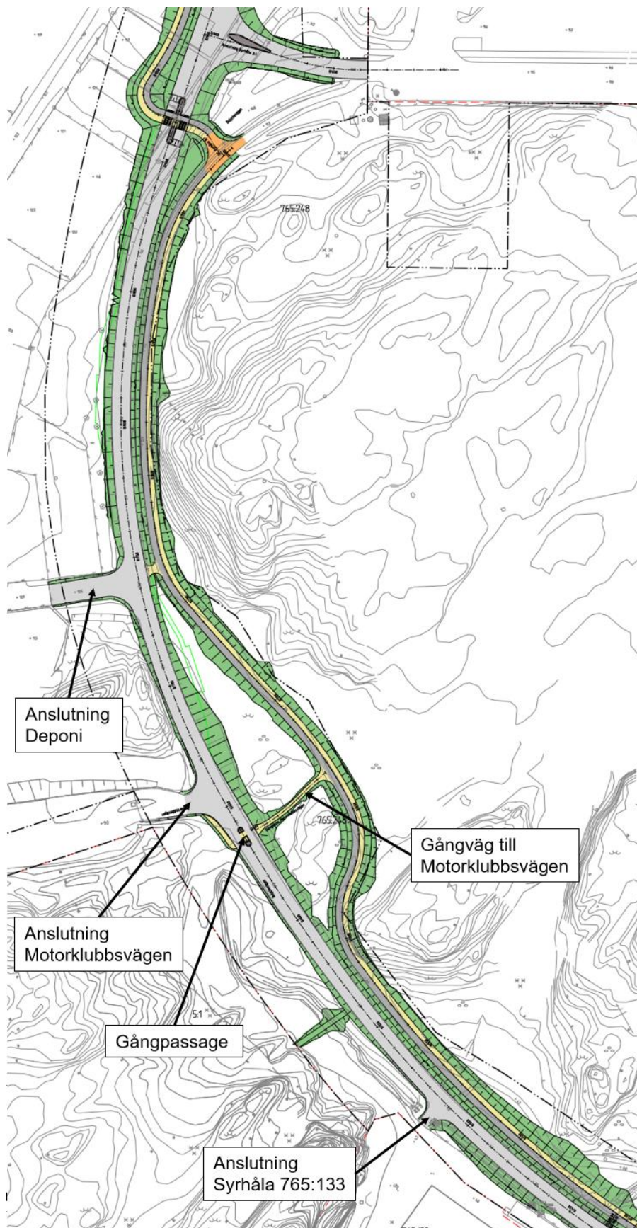
E.1:8 Planutformning 0/440-0/900.
