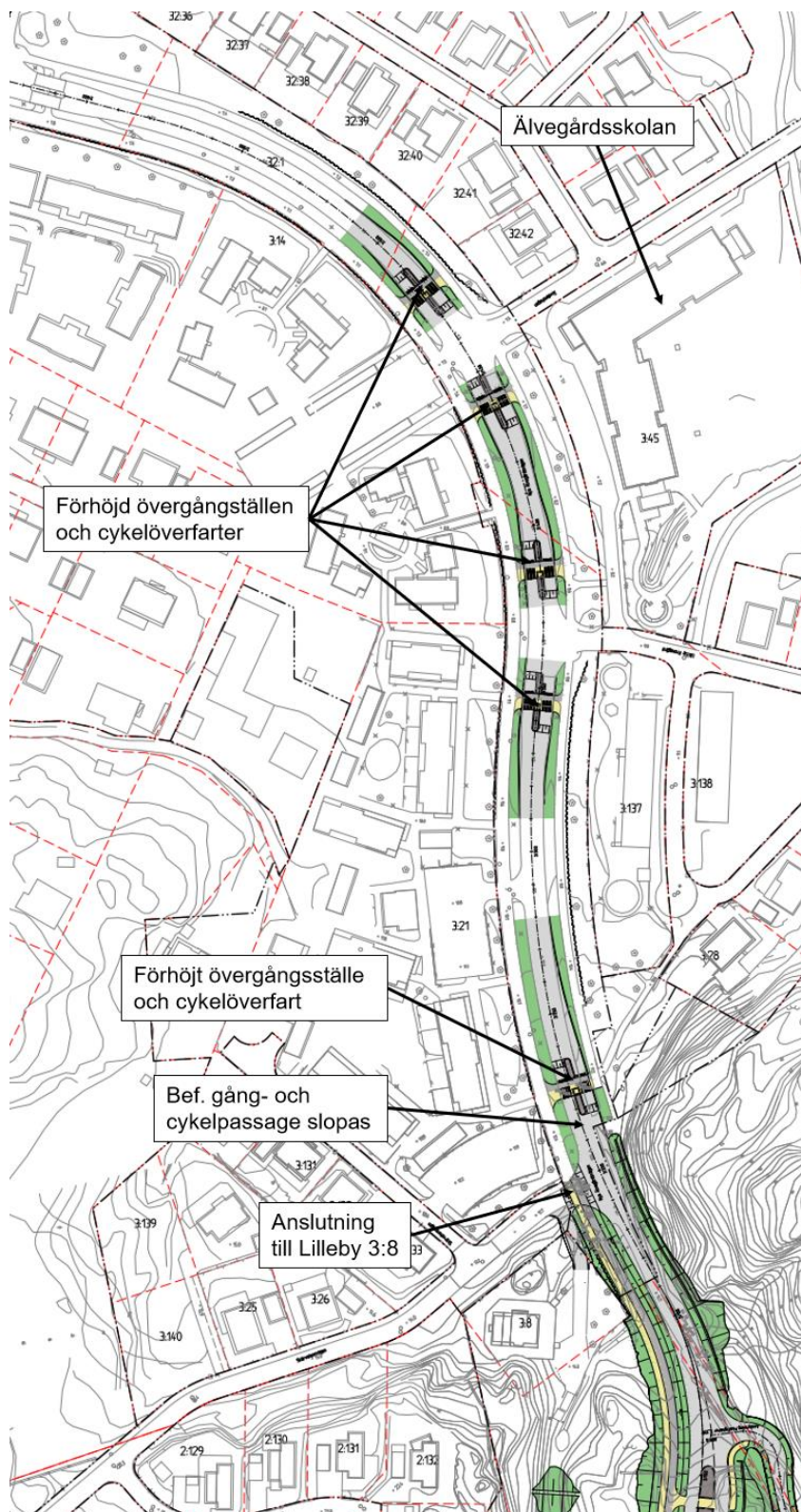
E.1:15 Planutformning 2/100-2/745.
