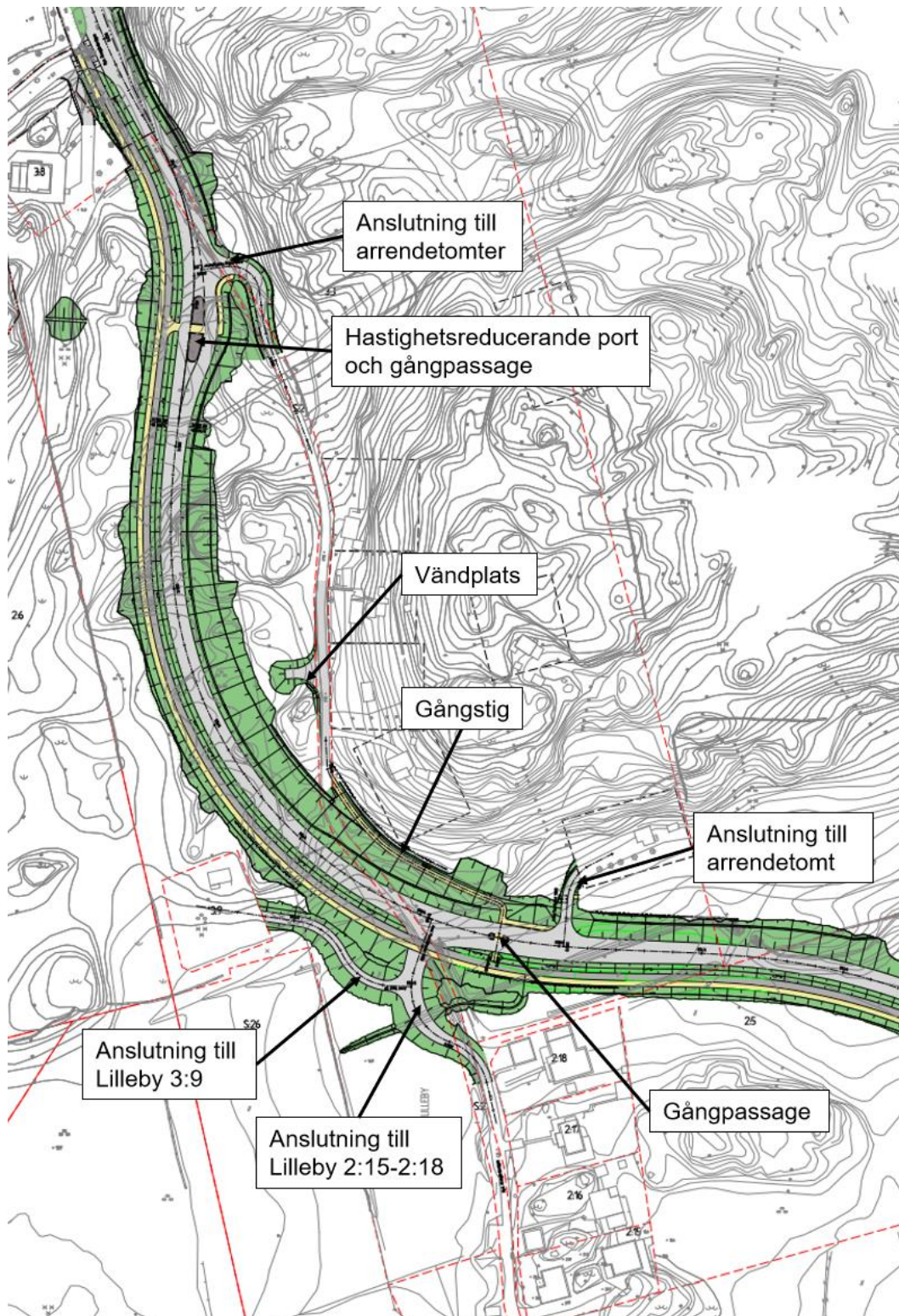
E.1:13 Planutformning 1/650-2/100.
